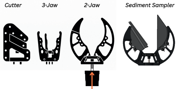
Threaded shaft enables attachment of various interchangeable heads.
