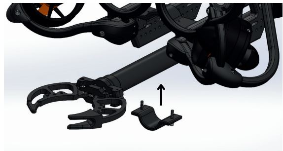
The Robotic Grabber Arm mounts securely to the underside of the ROV. Its position can be manually adjusted to extend the arm head as far out from the ROV as needed.
